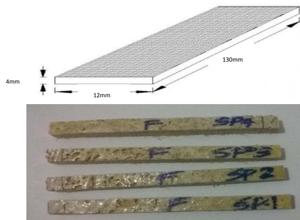
Fig 4.1 Tensile test specimens
