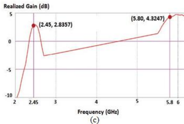
Fig. 5. (a) 3D radiation pattern at 2.45 GHz. (b) 3D radiation pattern at 5.8 GHz. (c) Simulated broadband realized gain across frequency (dB).
