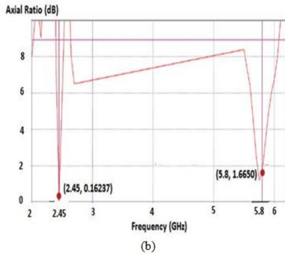
Fig. 3. (a) Measurement and simulated graph of S11. (b) Simulated axial ratio at 2.45 GHz and 5.8 GHz.
