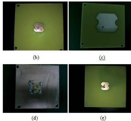
Fig. 1. (a) Overall antenna structure, (b) top patch (L1), (c) bottom patch (L2), (d) ground plane, (e) layout.
