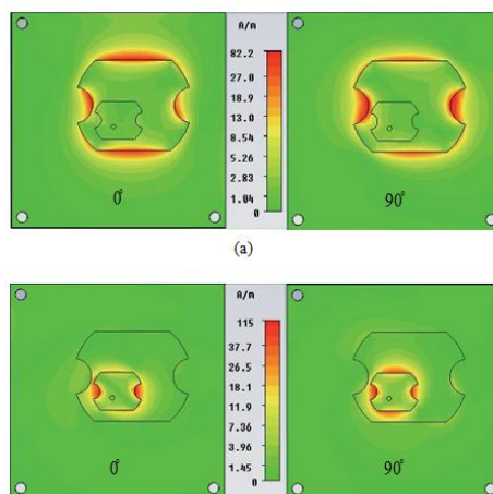
Fig. 2. Surface current distribution at (a) 2.45 GHz, (b) 5.8 GHz.
