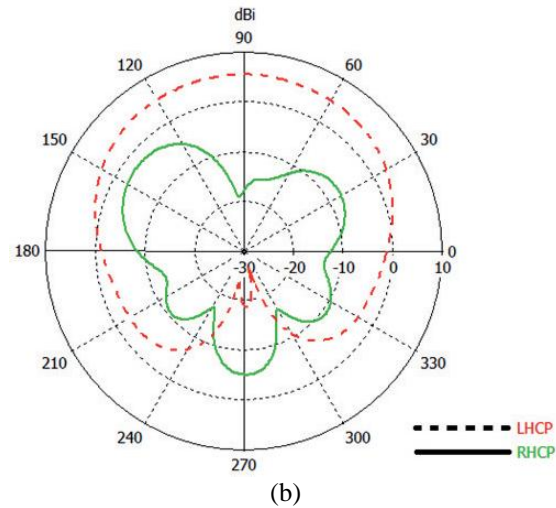
Fig. 4. (a) CP radiation pattern at 2.45 GHz. (b) CP radiation pattern at 5.8GHz.
