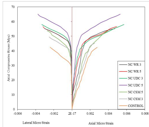
Figure 14. Stress-Strain Response for 0% Level of Corrosion-Damaged Columns
