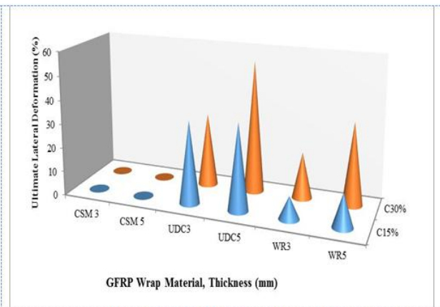
Figure 11. Effect of GFRP Wrap Material on Lateral Deformation of Corrosion-Damaged Columns
