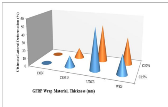
Figure 12. Effect of 3 mm Thick GFRP Wrap on Lateral Deformation of Corrosion-Damaged Columns
