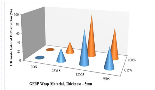
Figure 13. Effect of 5 mm Thick GFRP Wrap on Lateral Deformation of Corrosion-Damaged Columns
