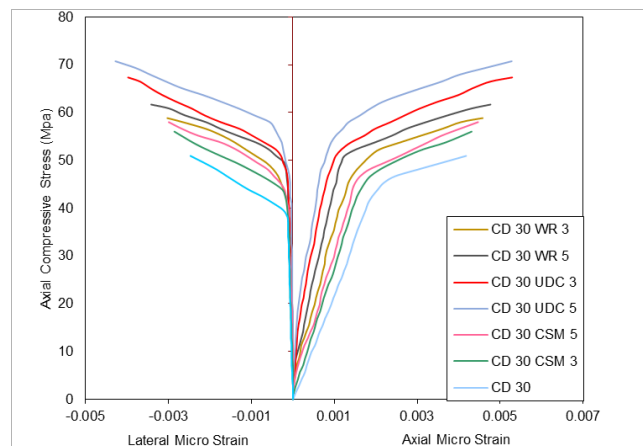
Figure 16. Stress-Strain Response for 30% Level of Corrosion-Damaged Columns
