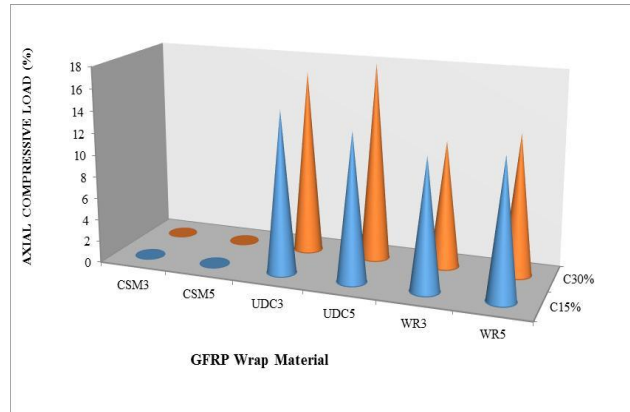
Figure 7. Effect of GFRP Wrap Material on Load Carrying Capacity of Corrosion-Damaged Columns Effect of GFRP Wrapping on Ultimate Axial Deformation
