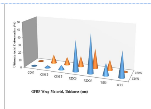
Figure 8. Effect of Various Levels of Corrosion-Damage on Axial Deformation of GFRP Wrapped Columns
