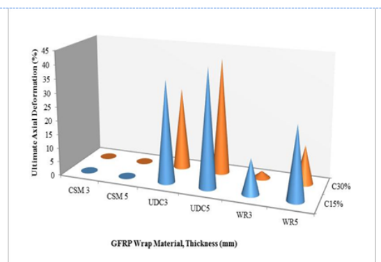
Figure 9. Effect of GFRP Wrap Material on Axial Deformation of Corrosion-Damaged Columns
