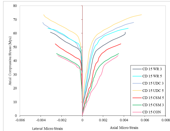
Figure 15. Stress-Strain Response for 15% Level of Corrosion-Damaged Columns
