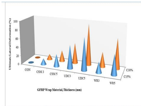
Figure 10. Effect of Various Levels of Corrosion-Damage on Lateral Deformation of GFRP Wrapped Columns
