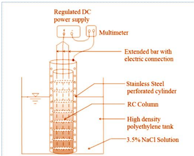
Figure.5: Schematic View of Accelerated Corrosion Set-up
