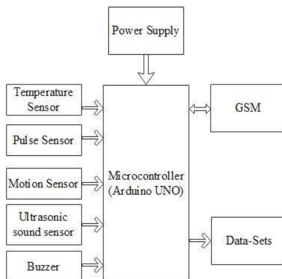
Fig -1: Architecture of Smart Wristband
