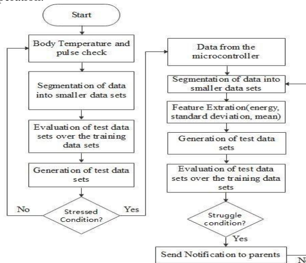
Fig -3: Methodology of Smart Wristband
