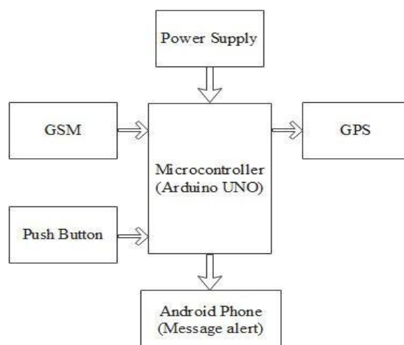
Fig -2: Architecture of Tracker Module
