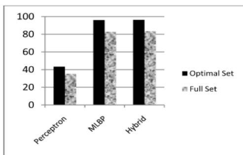
Fig. 4. Detection Rate percentage of the three types of neural networks using 8 and 38 features.
