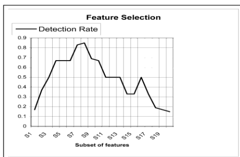
Fig. 2. Detection rate versus subset of features.
