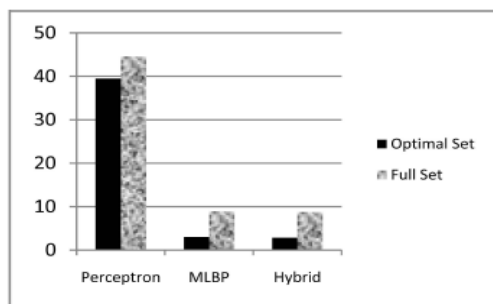
Fig. 5. False Positives Rate (%) for the three types of neural networks using 8 and 38 features.
