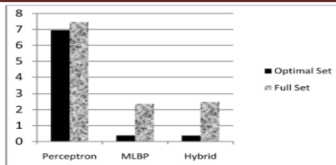
Fig. 6. False Negatives Rate (%) for the three types of neural networks using 8 and 38 features.
