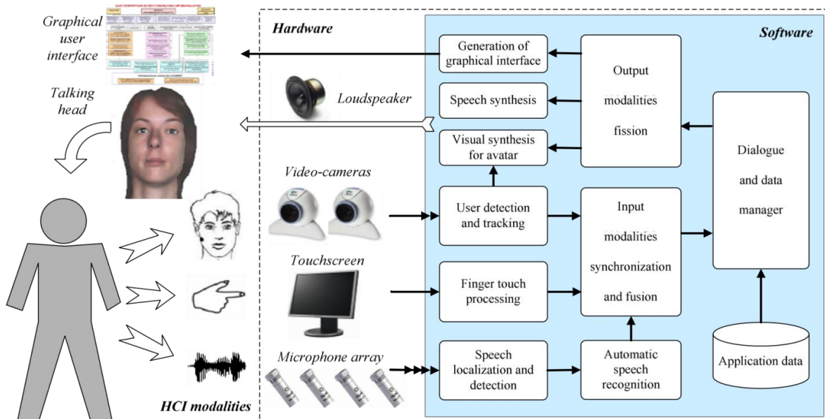
Figure 1. Hardware/software architecture of MIDAS intelligent information kiosk.
