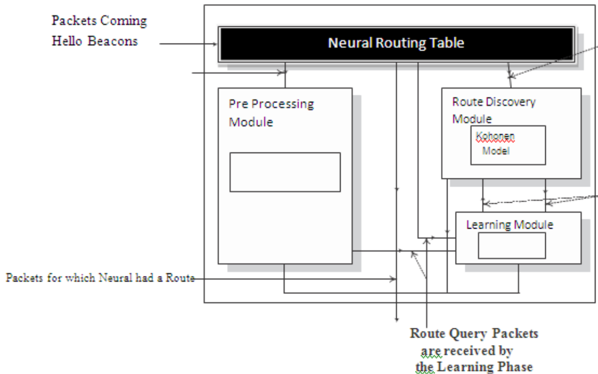
Figure 1. Schematic modular Architecture for NEURAL
